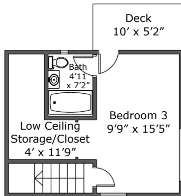
SECOND LEVEL
