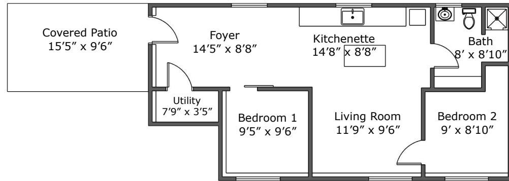
LOWER LEVEL
