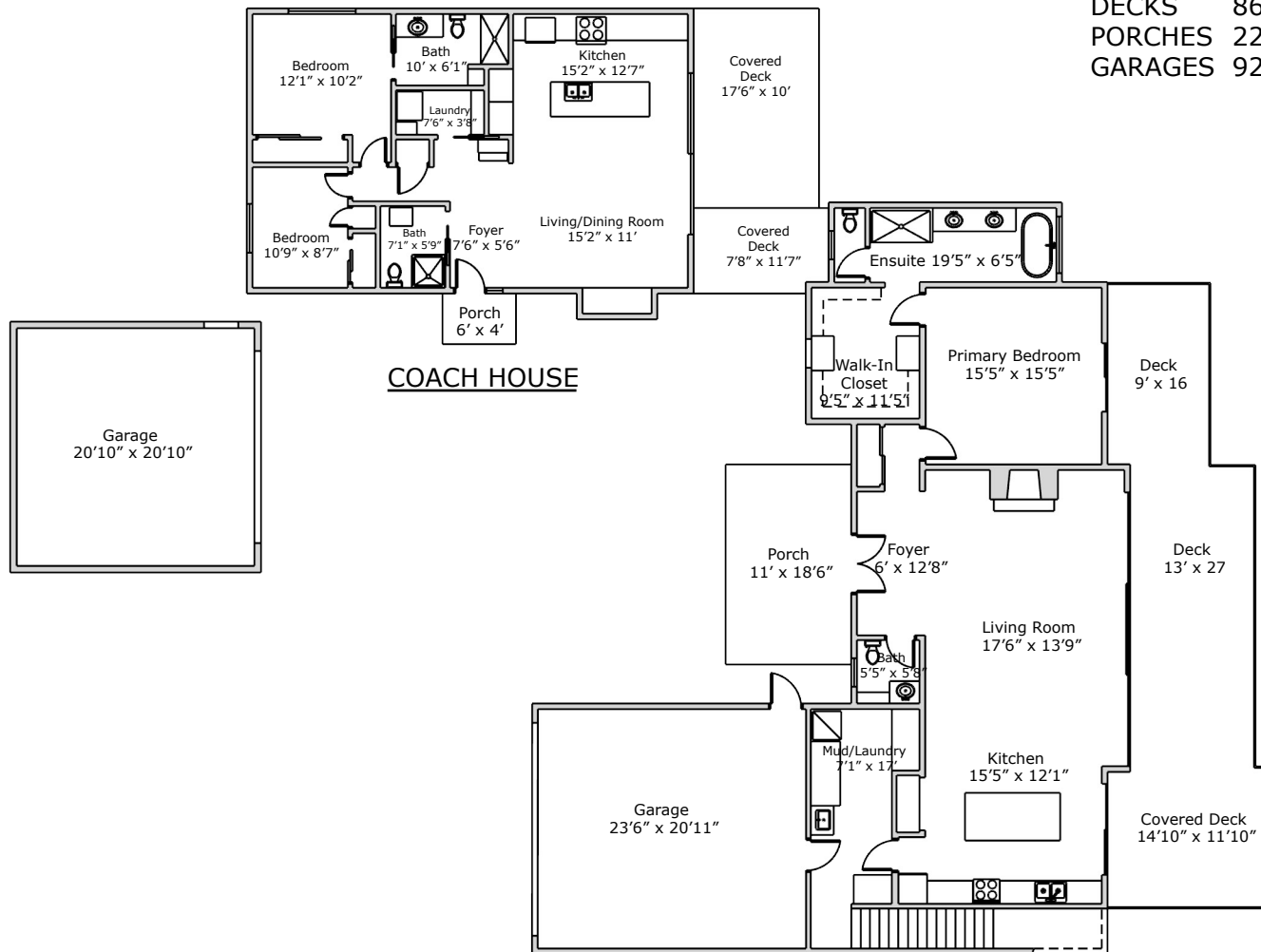
MAIN LEVEL
